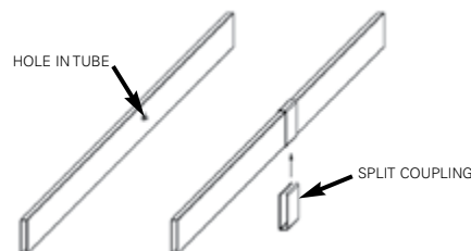
FIG. 30 Patching a hole in a tube
